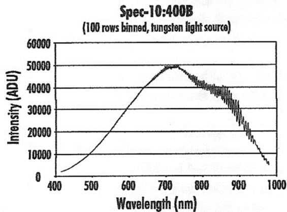
Figure 6. Spectrum of a tungsten light source using a back-illuminated CCD camera system. The etaloning becomes most pronounced between 800 nm and 1 \mu\text{m} , but is apparent even at 700 nm. ADU=arbitrary data unit.
