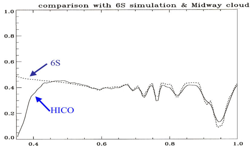
Comparison of smoothed 6S simulated apparent reflectance with HICO Apparent Reflectance
