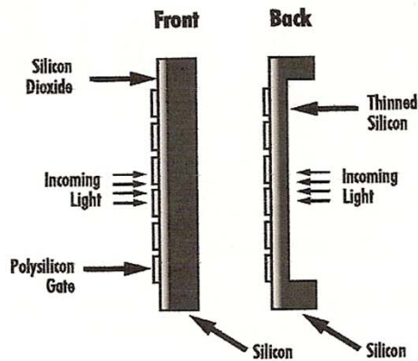
Figure 1. Comparison of front-illuminated and back-illuminated CCD.
