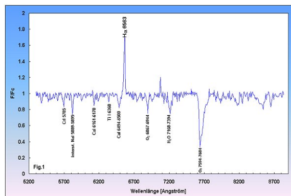
Fig.1: Resulting spectrum after data reduction as explained within the text.
