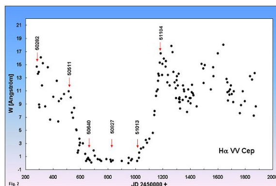
Fig. 2: Plot of W for H \alpha -emission as a function of time.
