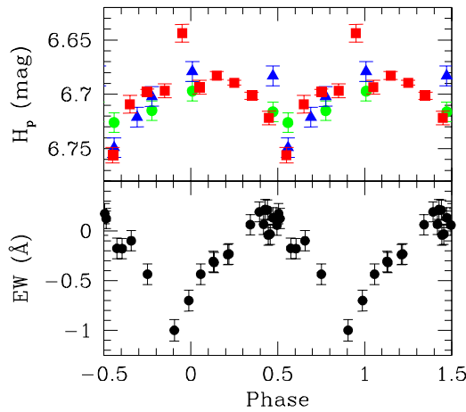
Figure 2: Top panel: Hipparcos light curve of HD 14134 binned to 0.1-phase resolution (squares). Our B - and I -band observations obtained in 2002 are overplotted as triangles and circles, respectively (the points are vertically shifted by a constant value to match the Hipparcos data). Bottom panel: EWs of the H\alpha line, as a function of phase. In all cases, the following ephemeris was used: \mathcal{P}=12.823 days and T_0=2,447,867.8 (zero phase arbitrarily set to maximum light). Adapted from Morel et al. (2004).
