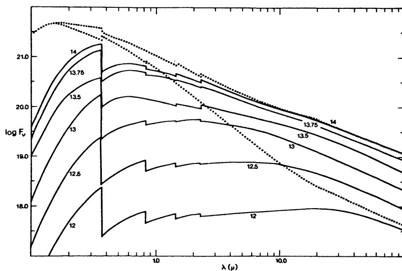
Figure 12. Continuum energy distribution for envelopes of various density (at 45^\circ inclination). Solid lines represent envelope emission (labelled in log density). Dotted lines represent the extremes for the total flux.
