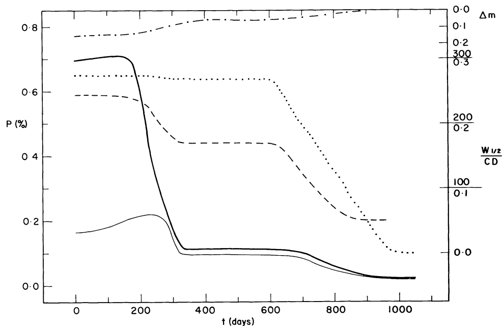
Figure 16. Polarization (light line, 3500A; heavy line 4000A), \Delta B (dot dash), H\gamma shell line depth (dots) and half width (dashed line) for the model as a function of time (days after start of density decrease).
