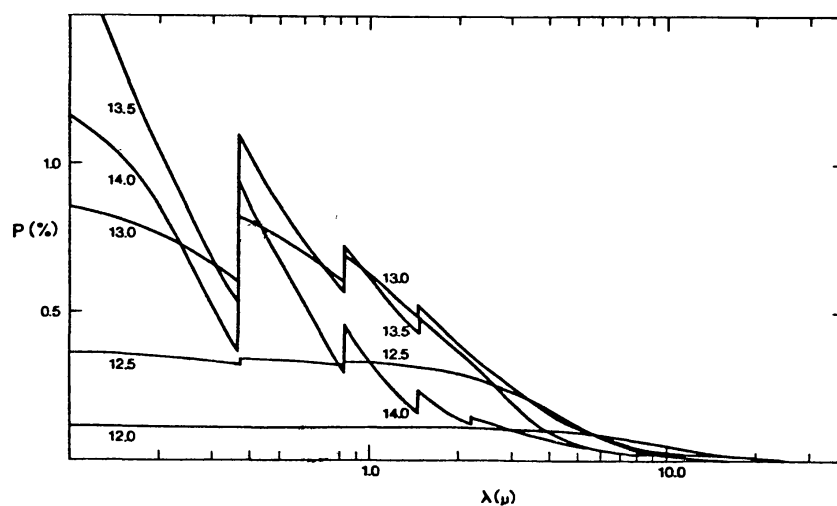
Figure 13. Continuum polarization for envelopes of various density (at 45^\circ inclination).
