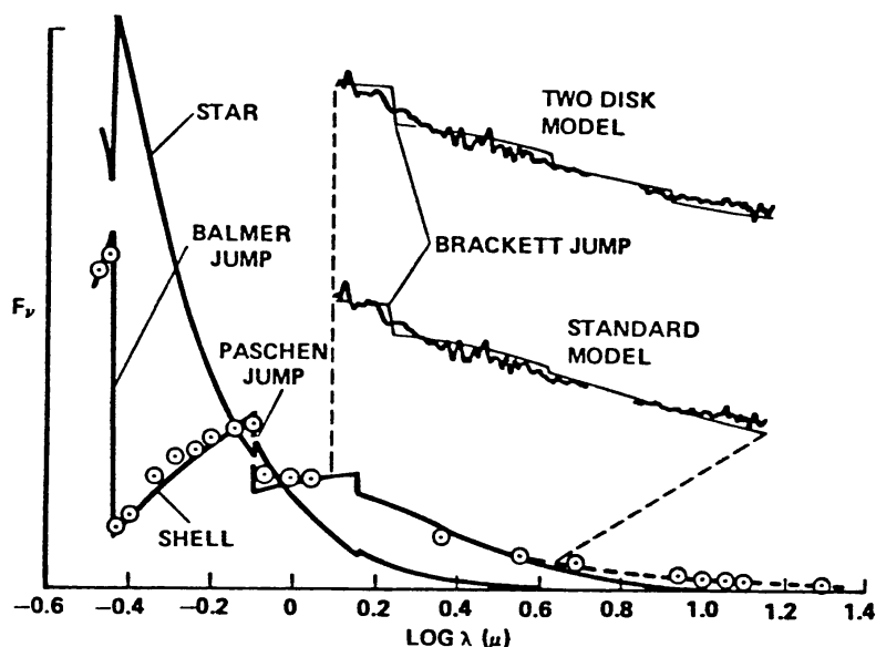
Figure 5. The flux excess (circles) and the model results for \gamma Cas. At 3751Å the shell contribution is 11% of the total flux.
